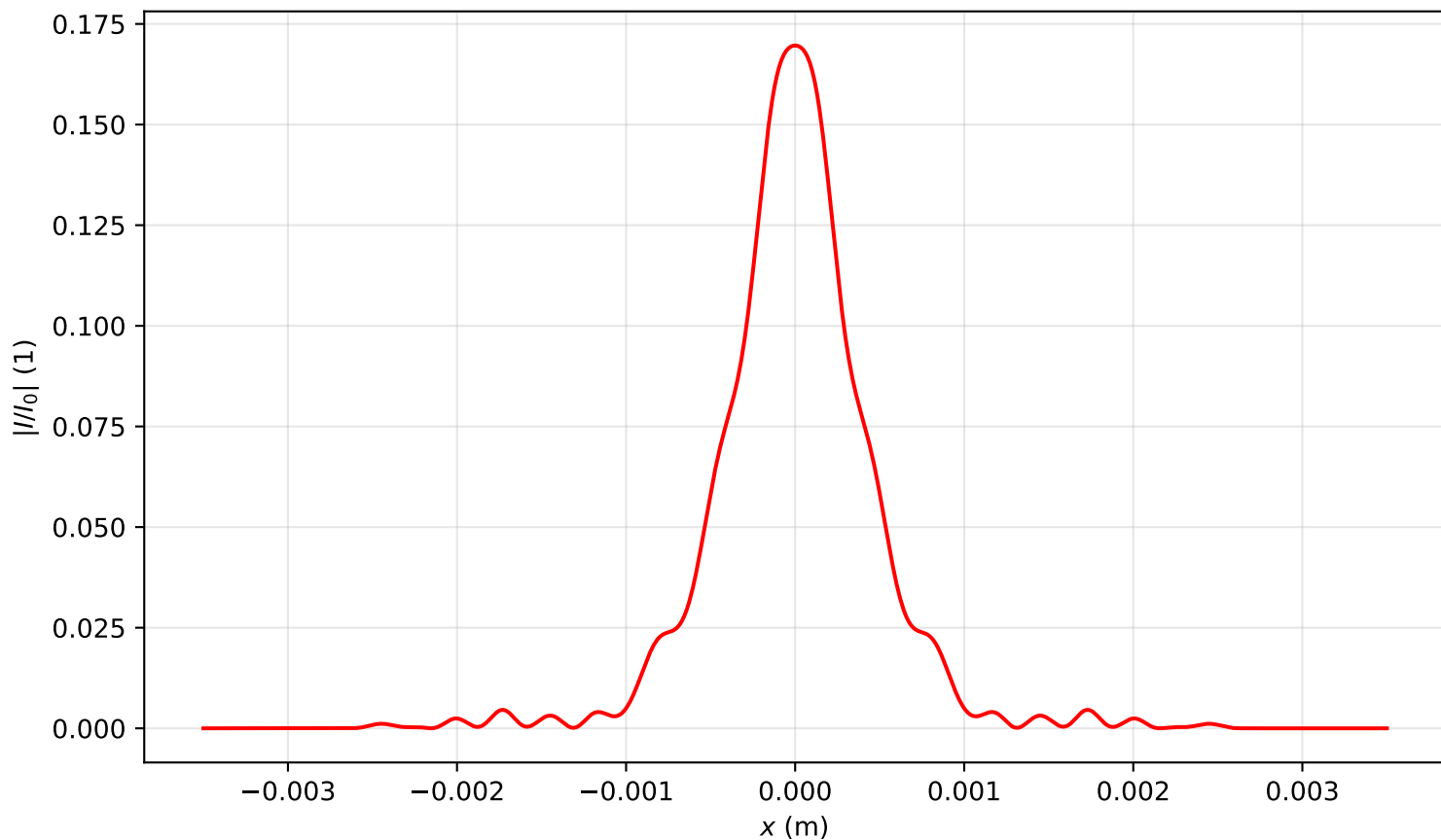
Intensity profile I(x, y = 0, z = 2.548)/I_0 , P_{in}=5.0P_{cr} , artificial time
